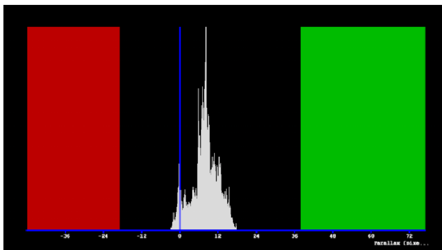
Parallax histogram.
